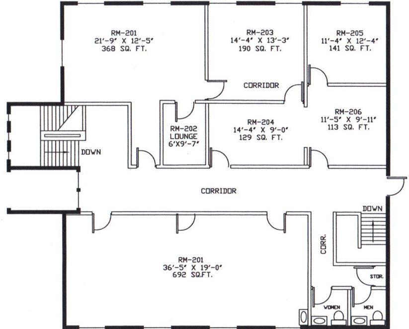
2ND FLOOR 2475 SQ. FT.
